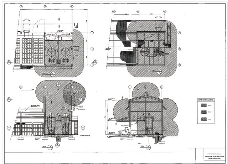
Fig. 2: Typical area classification of a surface plant where explosive vapours are present.
